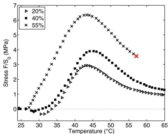
Figure 9. Stress vs. temperature during constrained recovery at 5 °C/min heating rate for samples pre-strained 20%, 40% and 55% at 40 °C during Step 1. [Color figure can be viewed in the online issue, which is available at wileyonlinelibrary.com .]
