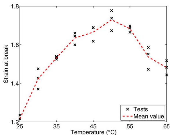
Figure 10. Strain at break with respect to temperature resulting from uniaxial tension tests run at a constant crosshead speed of 10 mm/min. 3-test mean values shown by the broken line. [Color figure can be viewed in the online issue, which is available at wileyonlinelibrary.com .]
