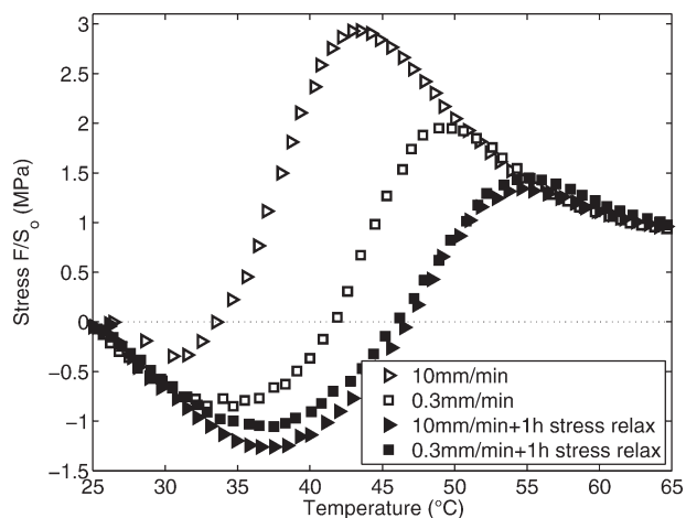
Figure 12. Stress vs. temperature during constrained recovery at 5 °C/min following various material stress relaxations during temporary 20% strain fixation at 40°C. Relaxation was permitted by slowing the loading strain rate and/or by allowing a stress relaxation of 1 h at 40°C after Step 1.
