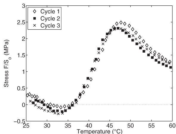
Figure 7. Step 4 constrained recovery during consecutive thermomechanical cycles for a sample pre-strained 20% at 45°C and heated at 5 °C/min.
