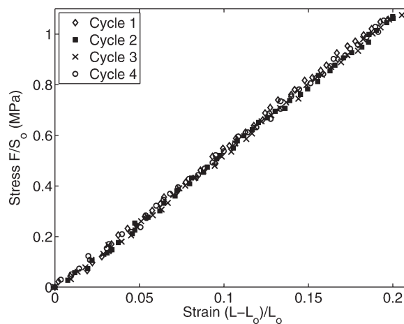
Figure 2. Material stress–strain response in uniaxial tension when deformed up to 20% at 65°C during Step 1 of four consecutive thermomechanical cycles.
