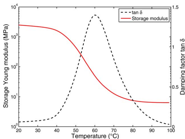
Figure 1. Dynamic mechanical analysis temperature sweep from 20°C to 100°C at 2 °C/min and 1 Hz. [Color figure can be viewed in the online issue, which is available at wileyonlinelibrary.com .]
